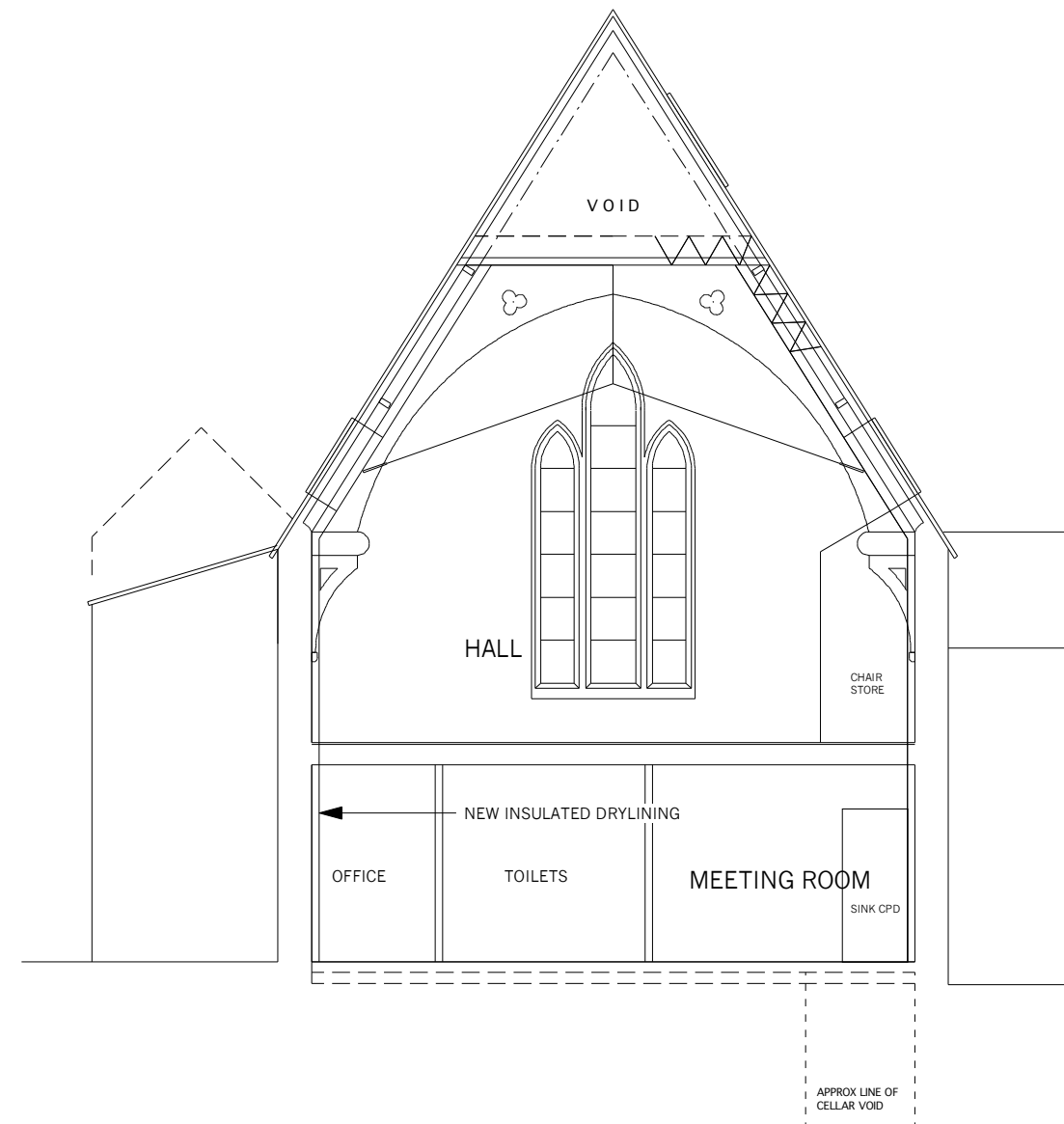
SECTION BB
